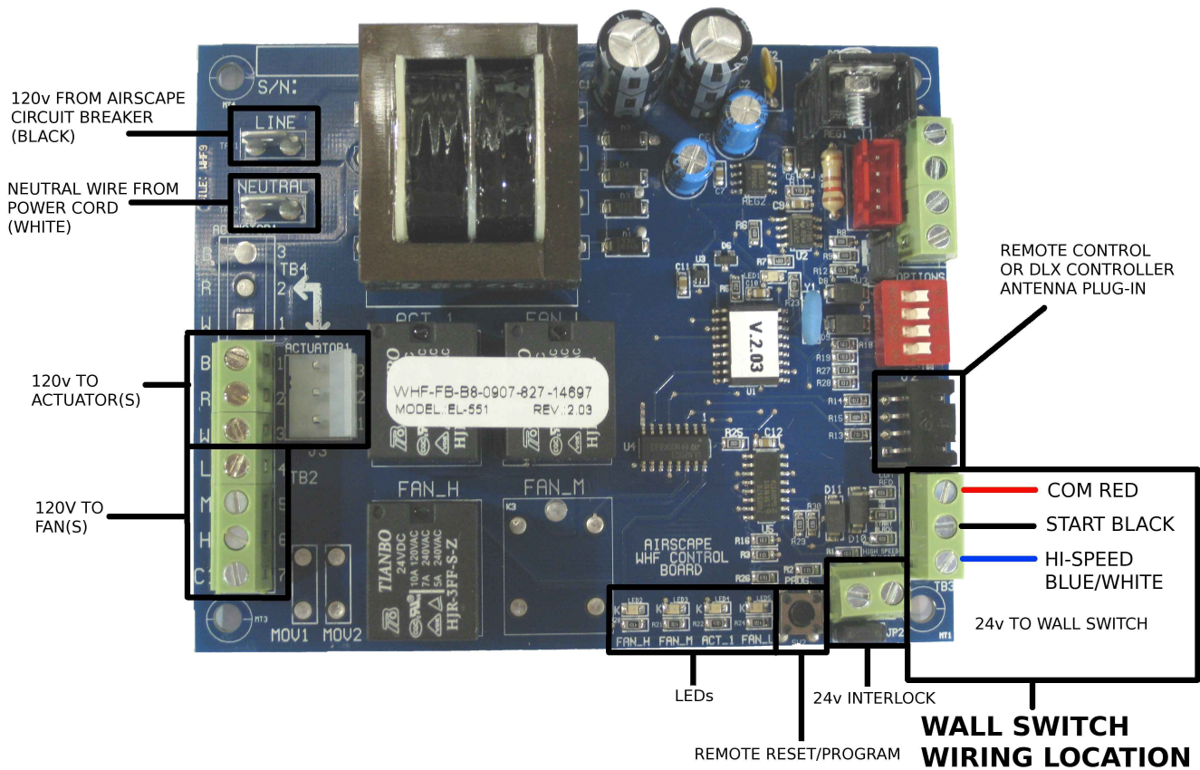
FIGURE 8 – Control Board Diagram
