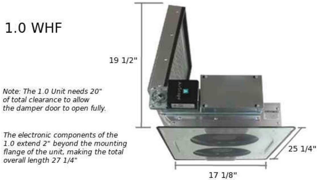
FIGURE 2 – 1.0/1.7 Dimensions
