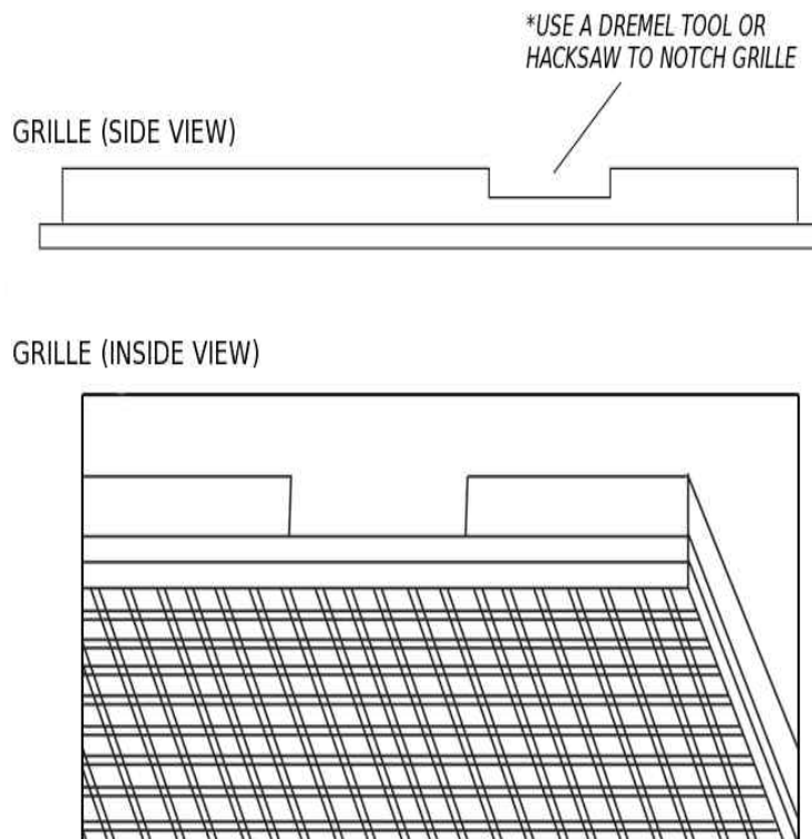
FIGURE 4 – Grille Notch -- ONLY 16" O/C Installations.
