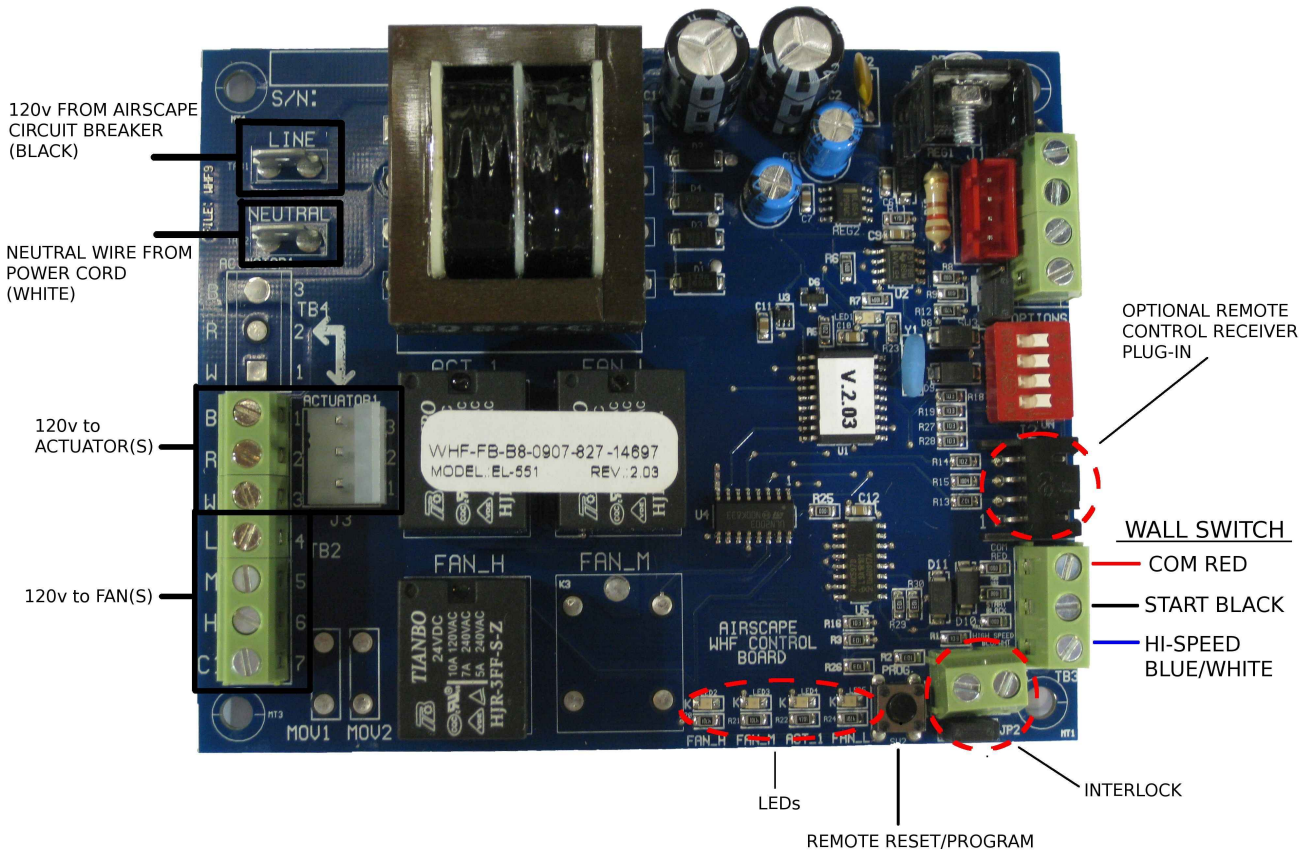
FIGURE 9 – Control Board Diagram
