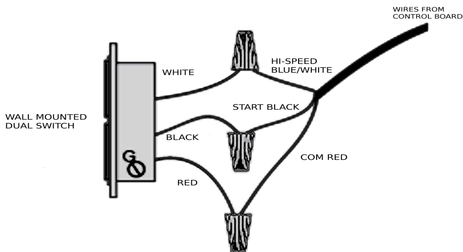
FIGURE 8 – Low Voltage Wall Switch Wiring
