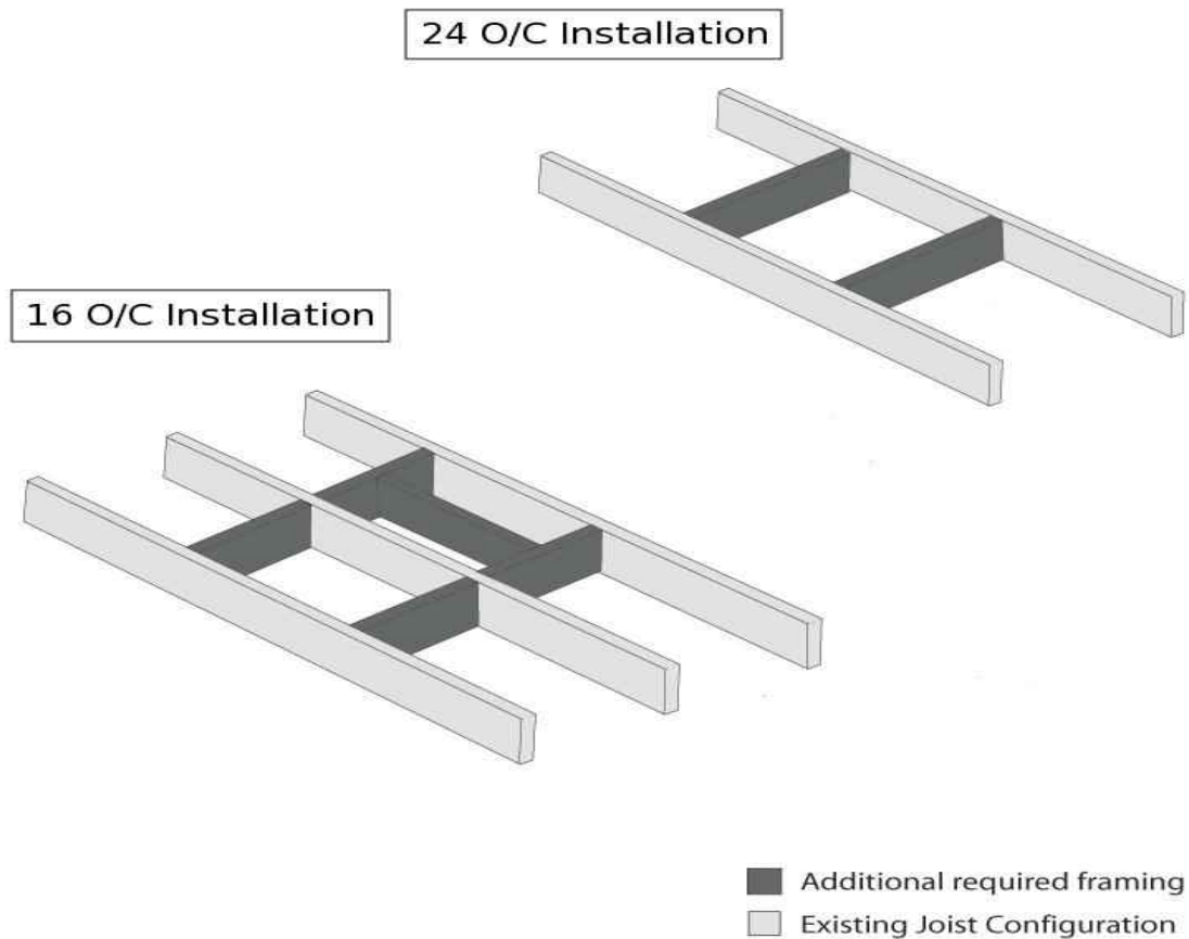
FIGURE 3 – Framing
