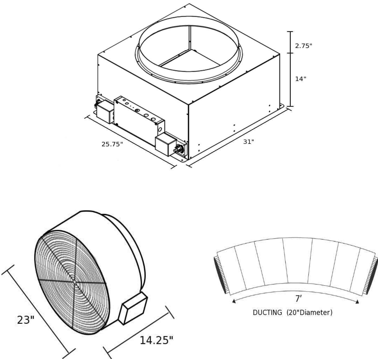
FIGURE 2 – Parts & Dimensions
