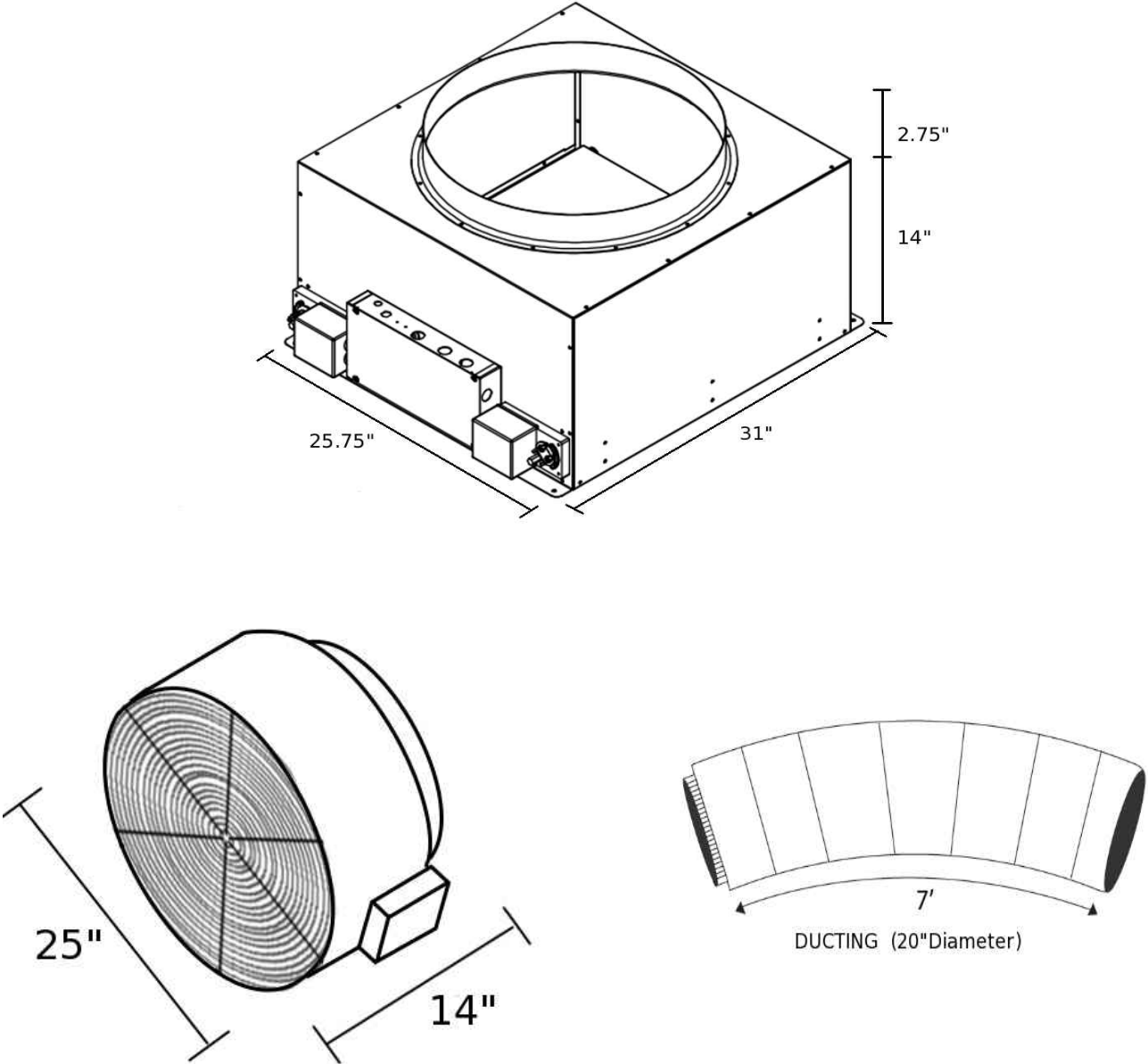
FIGURE 2 – Parts & Dimensions
