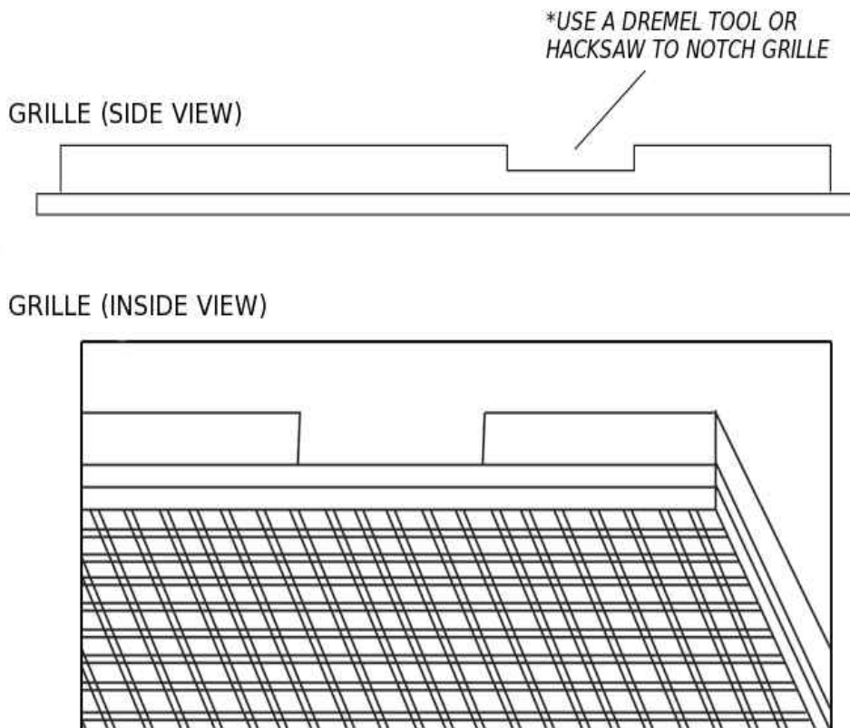
FIGURE 4 – Grille Notch – ONLY 16" O/C Installations.
