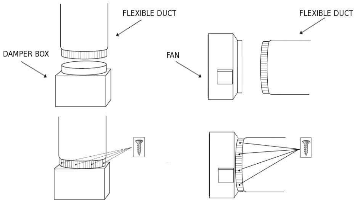
FIGURE 6 – Duct to Damper and Duct to Fan Connections
