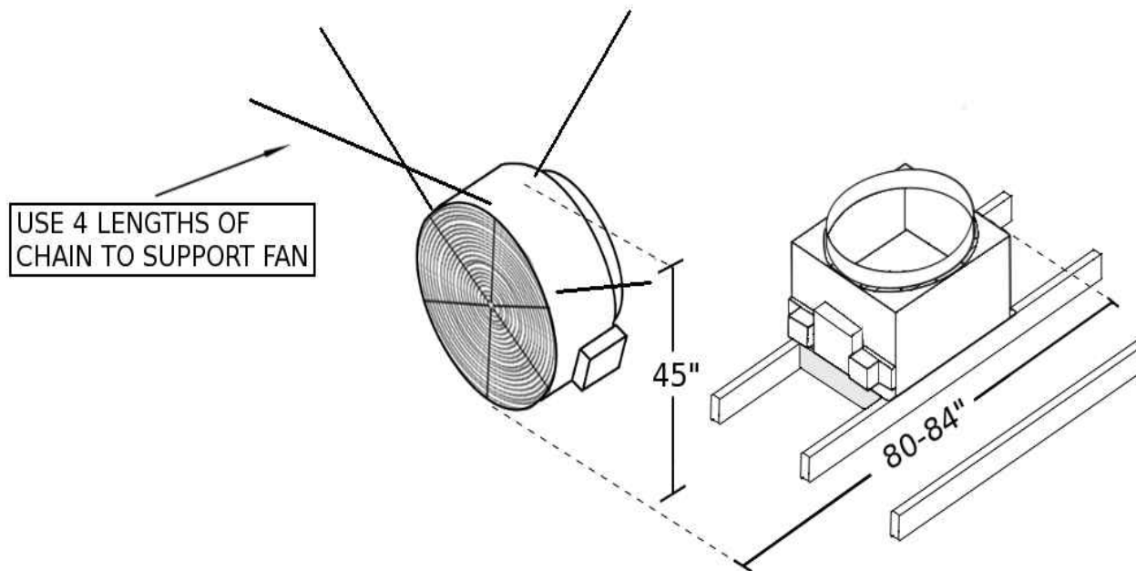
FIGURE 5 – Hanging the fan
