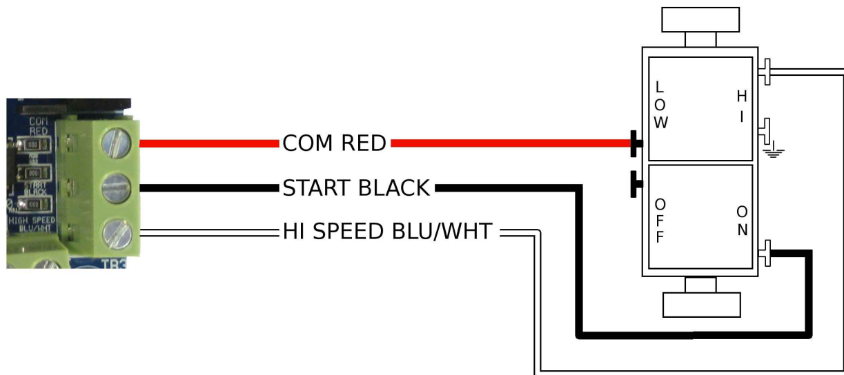
FIGURE 8 – Wall Switch Wiring
